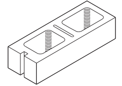
Half High Sash with Combo 5 5/8" x 3 5/8" x 15 5/8"
