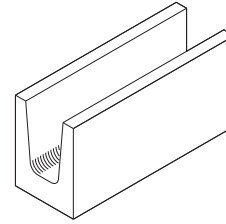
Bond Beam Solid 5 5/8" x 7 5/8" x 15 5/8"
