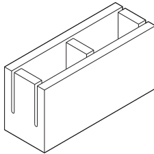
Bond Beam Knock Out 5 5/8" x 7 5/8" x 15 5/8"
