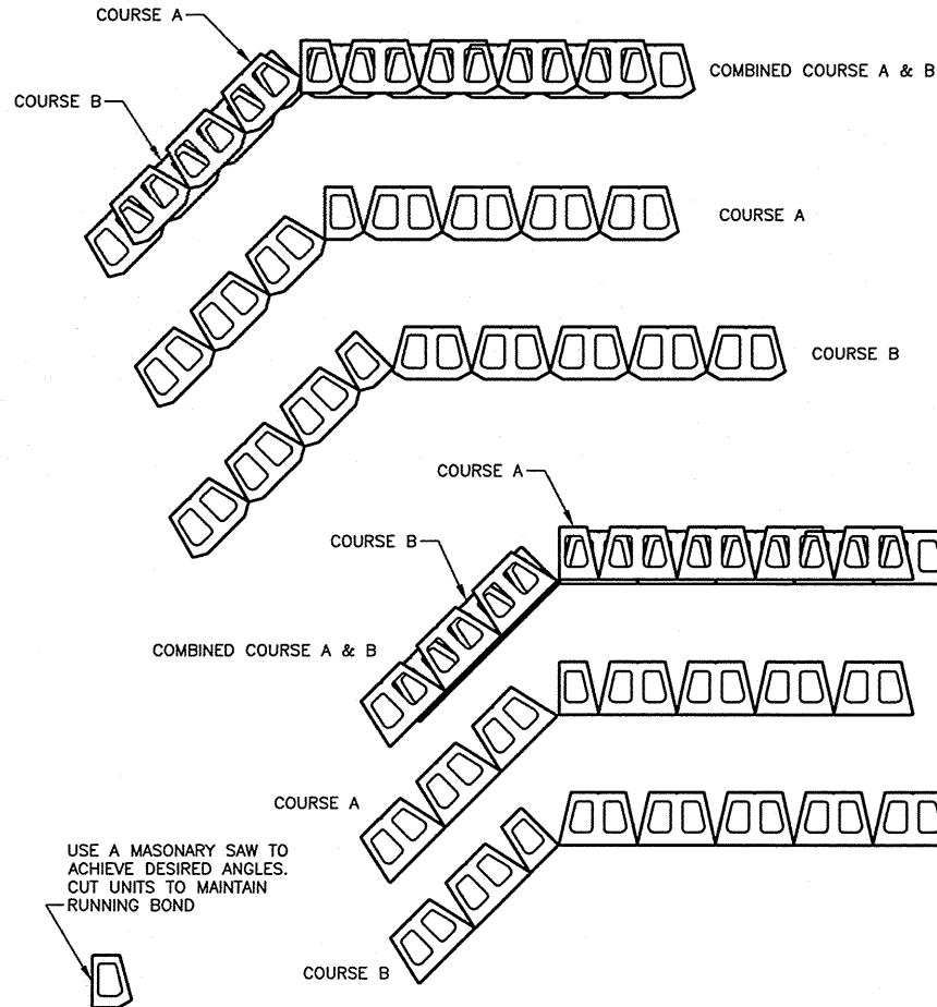
ANCHOR DIAMOND PRO™ X 45-DEGREE INSIDE CORNER (SCALE: 1/4" = 1'-0")
