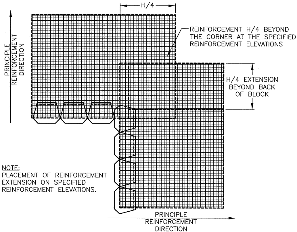
ANCHOR DIAMOND ® X 90-DEGREE INSIDE CORNER W/ GRID WX (NOT TO SCALE)
