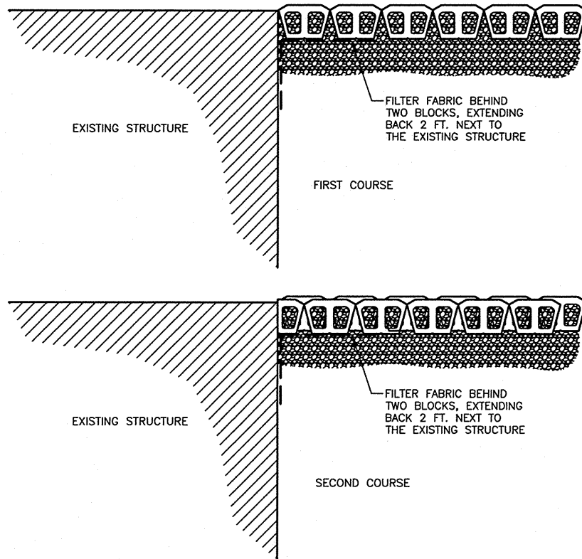
ANCHOR DIAMOND PRO™ WALL ABUTTING EXISTING STRUCTURE (X NOT TO SCALE)
