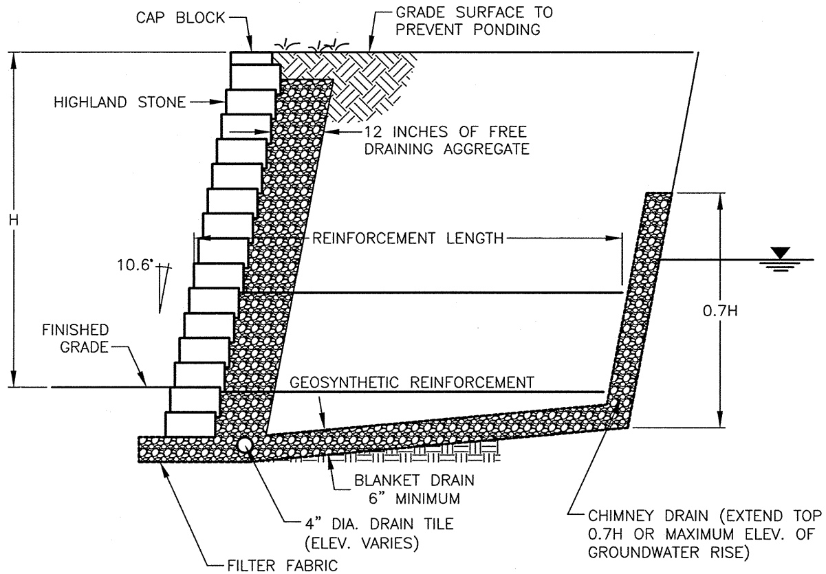
X WX ANCHOR HIGHLAND STONE™ POTENTIAL GROUNDWATER BEIND WALL (SCALE: 3/8" = 1'-0")
