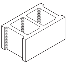
Stretcher 9 5/8" x 7 5/8" x 15 5/8"
