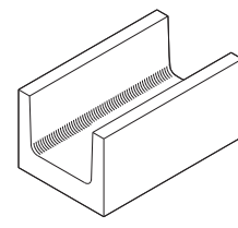
Bond Beam Solid 9 5/8" x 7 5/8" x 15 5/8"
