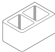
Double Bullnose on End 9 5/8" x 7 5/8" x 15 5/8"
