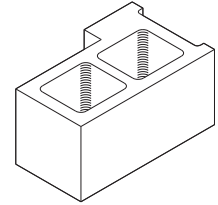
L-Corner 9 5/8" x 7 5/8" x 15 5/8"
